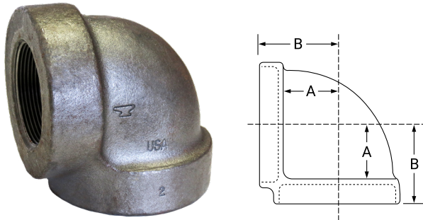
Fig. 421 90° Elbow (Class 250 Extra Heavy)
