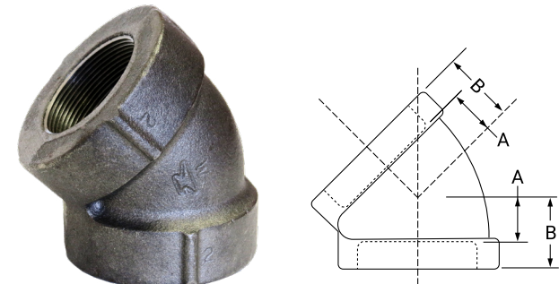
Fig. 424 45° Elbow (Class 250 Extra Heavy)
